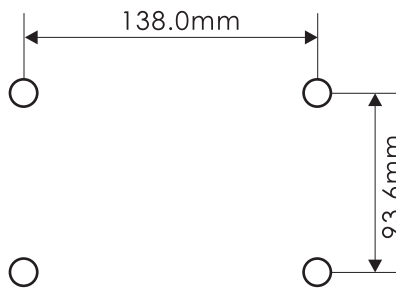
Installation Dimension
